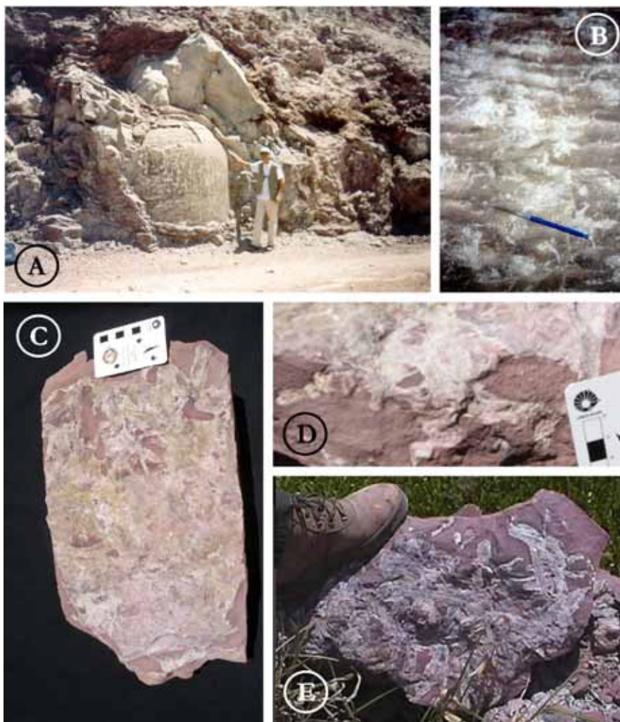
Figura 5 – Estromatólito gigante (A) associado a marcas de ondas (B) e icnofósseis (C, D e E) Figure 5 - A giant stromatolite (A) associated to ripple marks (B) and icnofossils (C, D and E)
